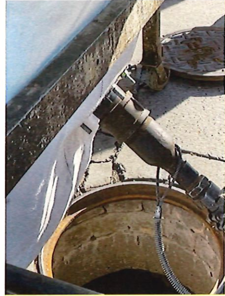
Figure 3: View of liner material being prepped in the inversion machine
