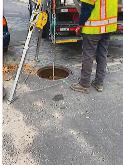
Figure 3: View of attendant at manhole while debris is removed by occupant
